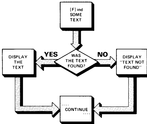
Figure 6-2. Conditional Execution
